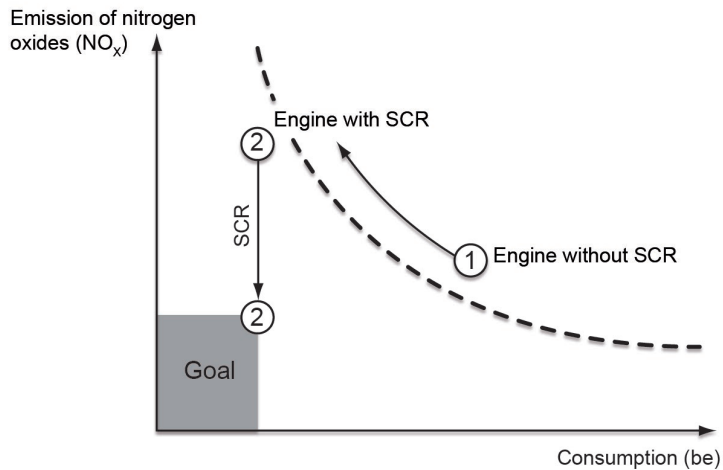
Fig. 3: Diagram of fuel consumption and nitrogen oxide emissions relationship High combustion temperatures result in economical fuel consumption, but also to high levels of nitrogen oxide. A SCR system can subsequently remove up to 90 percent of the nitrogen oxide produced during the combustion process from the exhaust gas.
