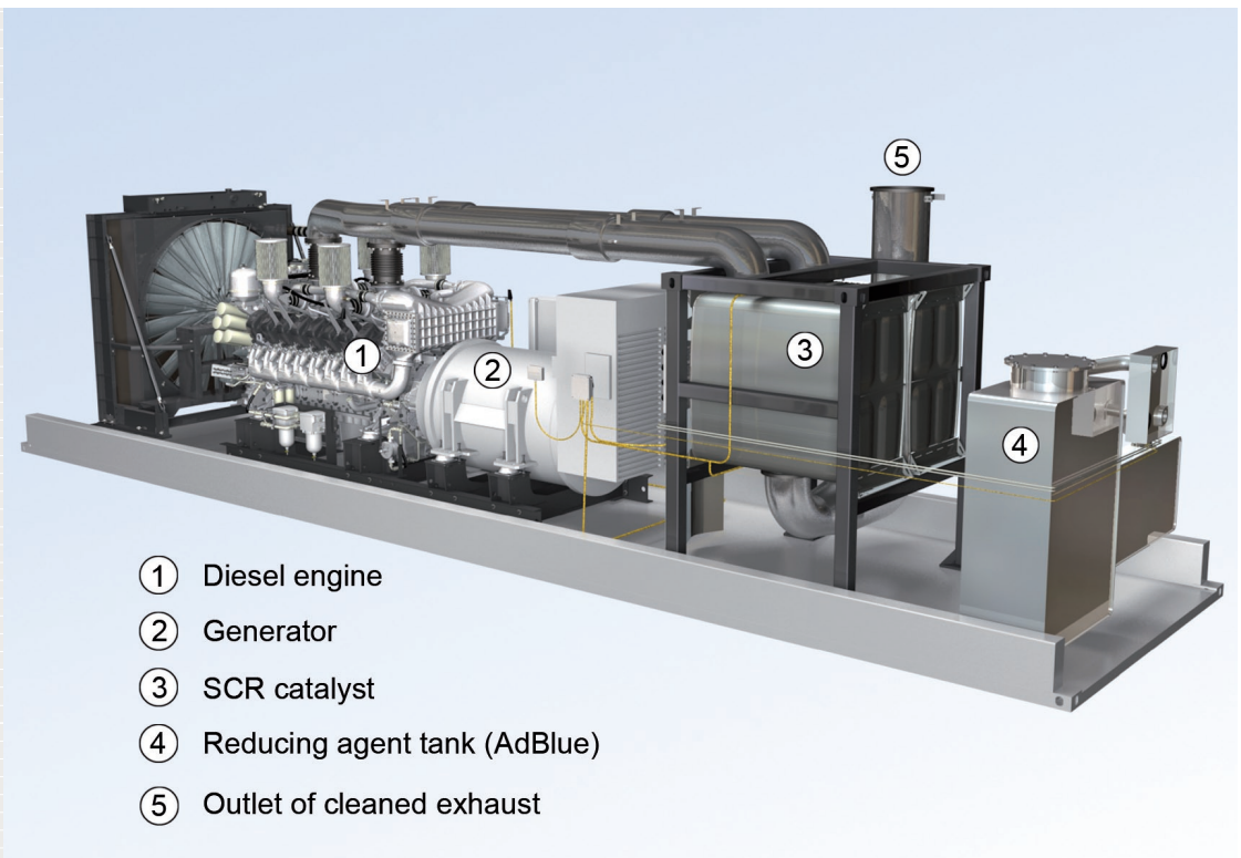
Fig. 2: Genset with a 16 cylinder Series 4000 engine equipped with SCR system
