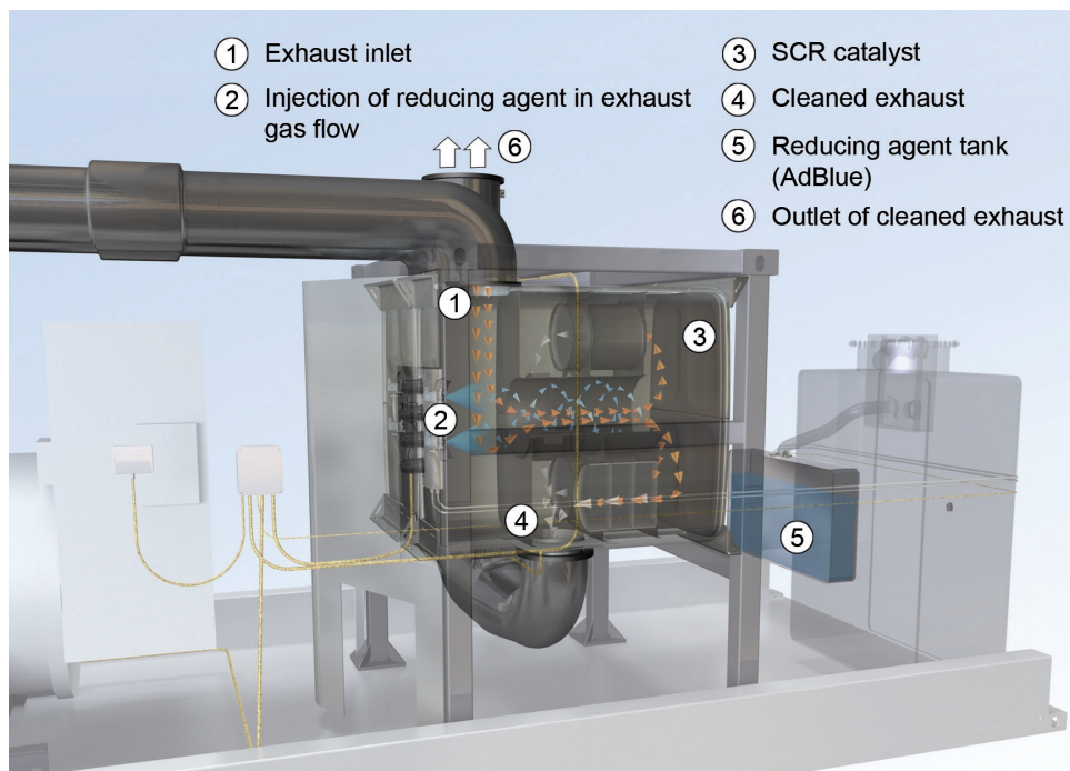
Fig. 4: Schematic of the operating principle of the SCR system In the SCR catalytic converter, ammonia converts the nitrogen oxides into water vapor and nitrogen. For this purpose, a reducing agent is continually injected into the exhaust gas flow using a metering module. In the exhaust gas flow, the fluid reacts within a fraction of a second to produce ammonia. This chemical compound then converts the nitrogen oxides in the SCR catalytic converter.
